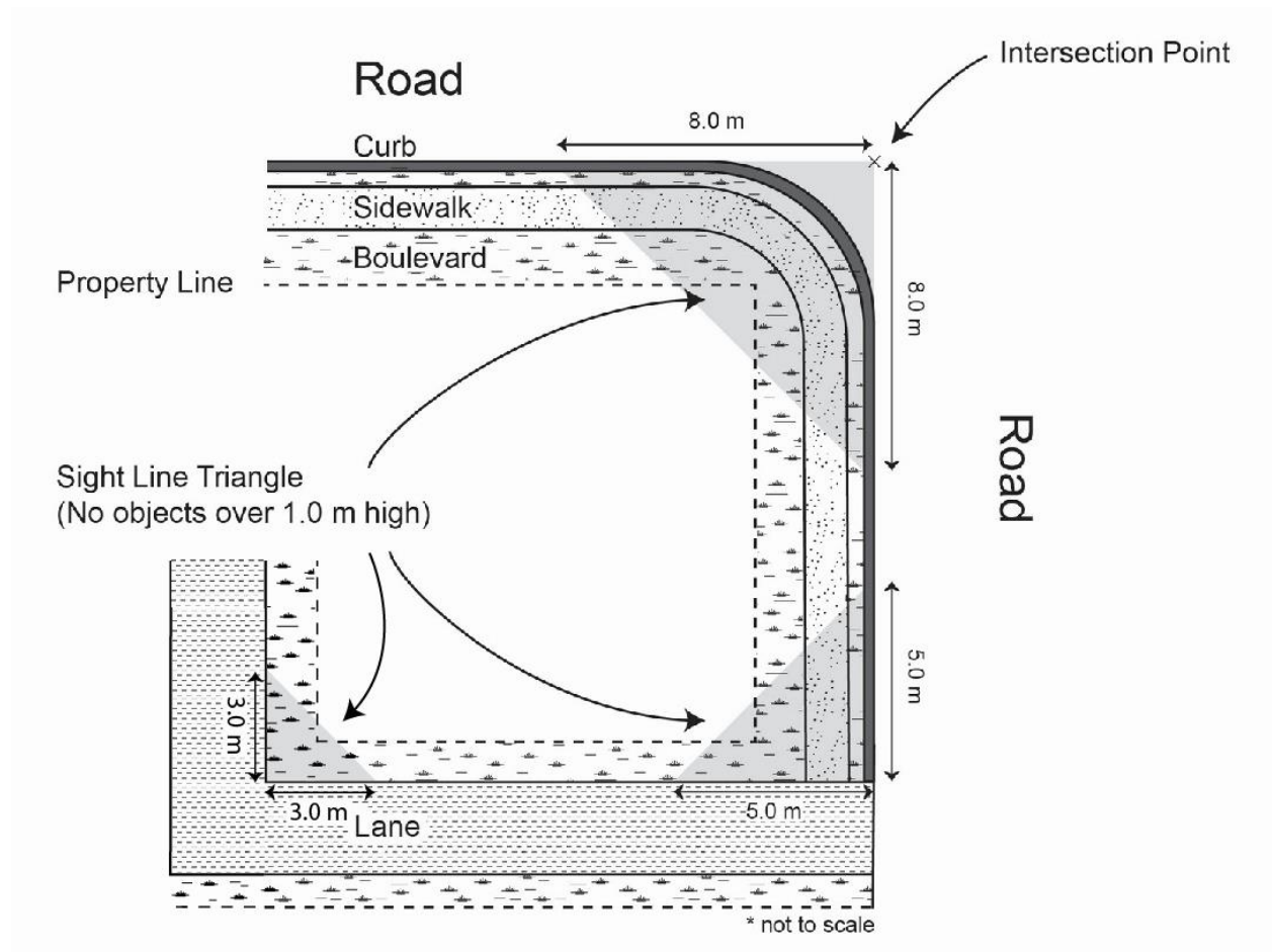
Figure 3.6.1. – Sight Line Triangle
